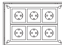
VL.BT.06 200 × 280 mm* chasing for 6 cavity sockets d = 68 mm, example configuration right
