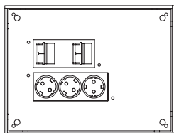
VL.BT.03 240 × 320 mm* triple power socket quadruple data socket
