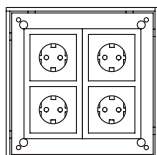
VL.BT.05 200 × 200 mm* chasing for 4 cavity sockets d = 68 mm, example configuration right
