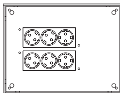
VL.BT.04 240 × 320 mm* 2 x triple power socket
