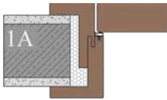
Frame system (1A) INTRA 63-75 TS40 Jamb and casing mounted on the wall Split jamb Casing widths 63mm / 75mm
