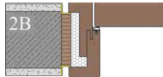
Frame system (2B) INTRA UZ-ALU 40-52 TS40 Jamb and casing flush with the wall split jamb with sub-frame and aluminum wall finishing strips Casing widths 40/52mm
