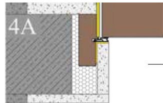
Frame system (4A) FLAT VD Concealed block jamb with aluminum protective profile
